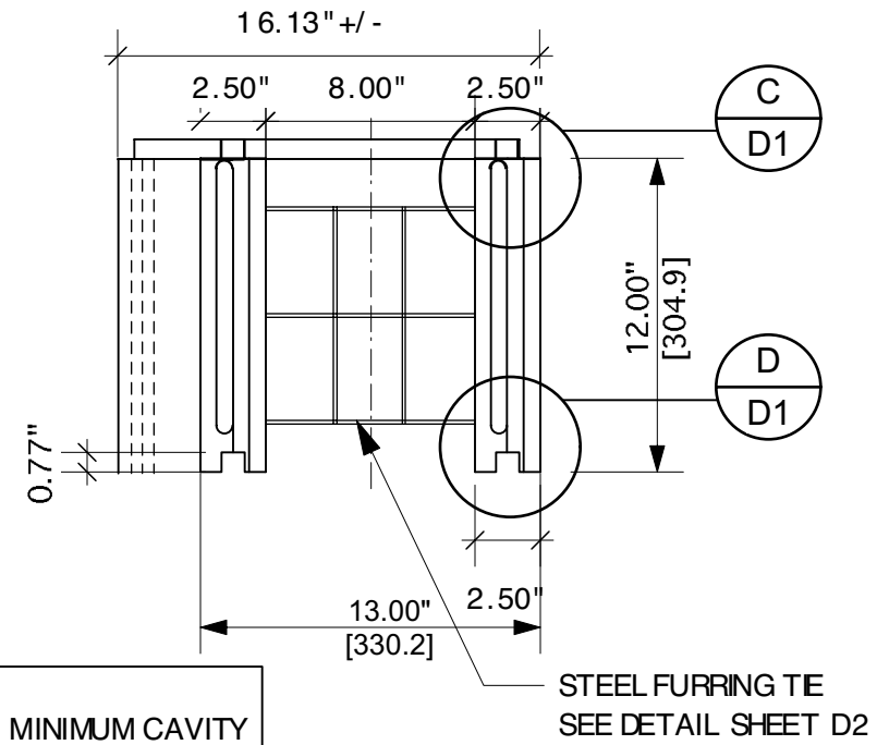
END ELEV,
