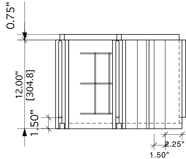
FRONT ELEV,
